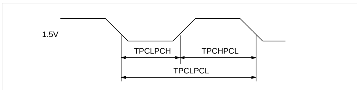
Figure 5.3 IMS T400 ProcClockOut timing
