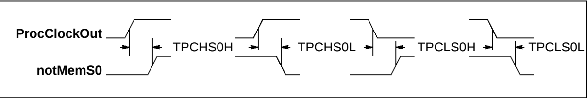
Figure 5.7 IMS T400 skew of notMemS0 to ProcClockOut
