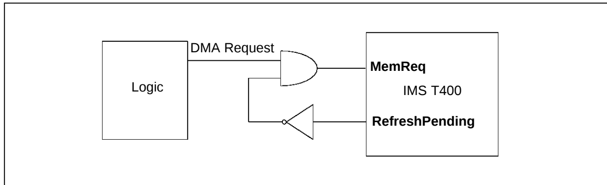
Figure 5.10 IMS T400 refresh with DMA
