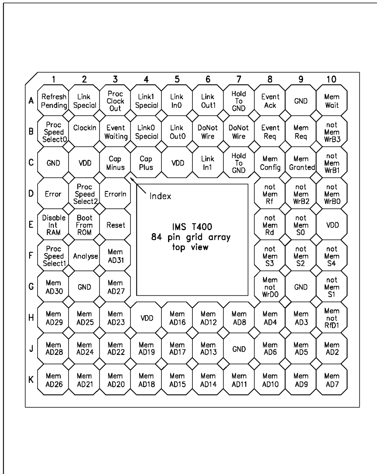
Figure 9.1 IMS T400 84-pin PGA package pinout
