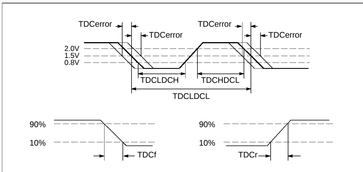
Figure 3.2 ClockIn timing
